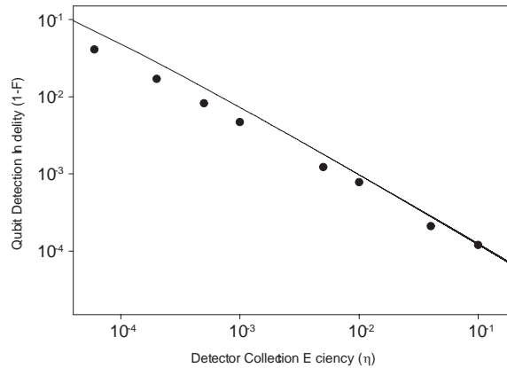
Fig. 5. Theoretical prediction of detection infidelity ( 1-F ) using the P_{3/2} detection scheme for ^{111}\text{Cd}^+ as a function of total detector collection efficiency ( \eta ). Filled circles are numerically calculated using eqn. 17 with iterations to find the optimal light level & detection time for each \eta ; solid curve uses the approximate analytic result of eqn. 19.
