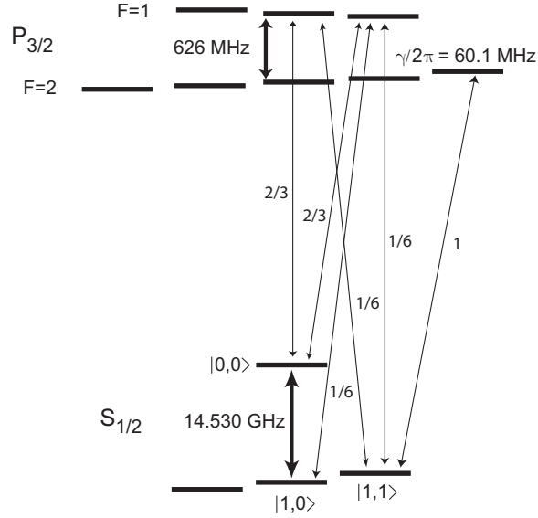
Fig. 3. Relevant energy level spacings and relative electric dipole strengths for selected transitions in ^{111}\text{Cd}^+ [33, 34, 35]. Note that the Zeeman splitting ( < 10 MHz) is small compared to the hyperfine splittings.
