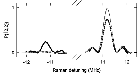
FIG. 2. Raman absorption spectrum of a single ^9\text{Be}^+ ion after Doppler precooling (solid points) and after five cycles of additional resolved sideband stimulated Raman cooling on the x dimension (hollow points). The observed count rate is normalized to the probability P\{|2, 2\rangle\} of the ion being in the |2, 2\rangle state. The first blue and red sidebands of the x dimension are shown at \delta_{pr}/2\pi \approx \pm 11.2 MHz. Similar sidebands are found near \pm 18.2 MHz ( y dimension) and at \pm 29.8 MHz ( z dimension). For precooling, the asymmetry in the sidebands indicates a thermal average vibrational occupation number of \langle n_x \rangle \approx 0.47(5) . For Raman cooling, the reduction of the red sideband and growth of the blue sideband implies further Raman cooling in the x dimension to \langle n_x \rangle \approx 0.014(10) . The widths of the features are consistent with the 2.5 \mu\text{s} Raman probe time. Each point represents an average of 400 measurements, corresponding to \approx 5 min of integration time for the entire data set. The lines connect the data points.
